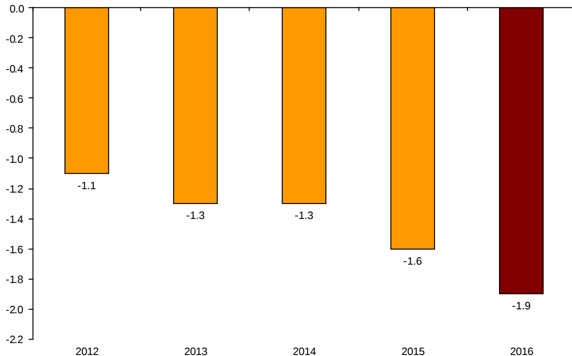
Evolution of the monthly rate of the CPI in the month of January
